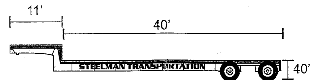
Stepdeck or Dropdeck Trailer
