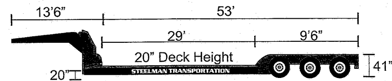
Removeable Gooseneck or RGN
