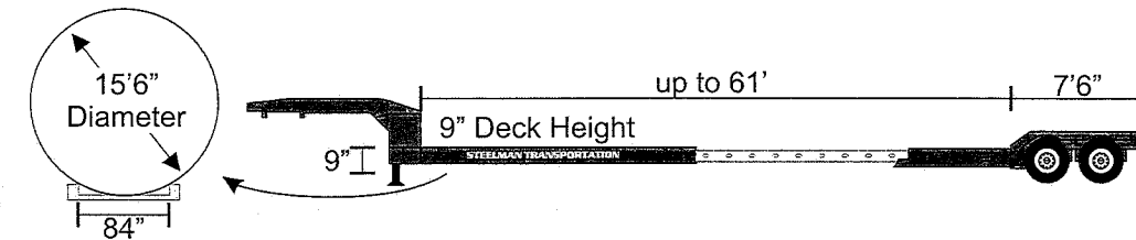
Perimeter Frame Rail Design Trailer
